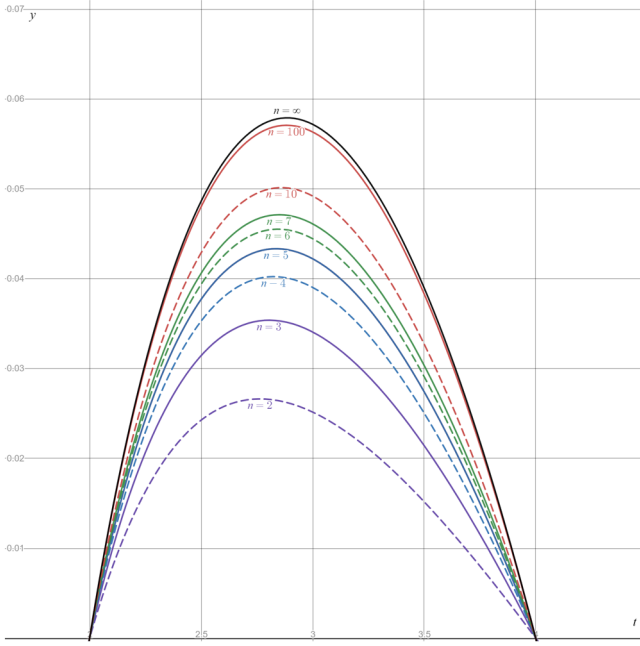
Fig. 7. Graphs of f_n(t) for selected values of n . Our numerical experiments indicate that, for all t \in [2, 4] , f_n(t) increases monotonically to f_\infty^*(t) := 1 - \frac{2^{1/2}}{t}
