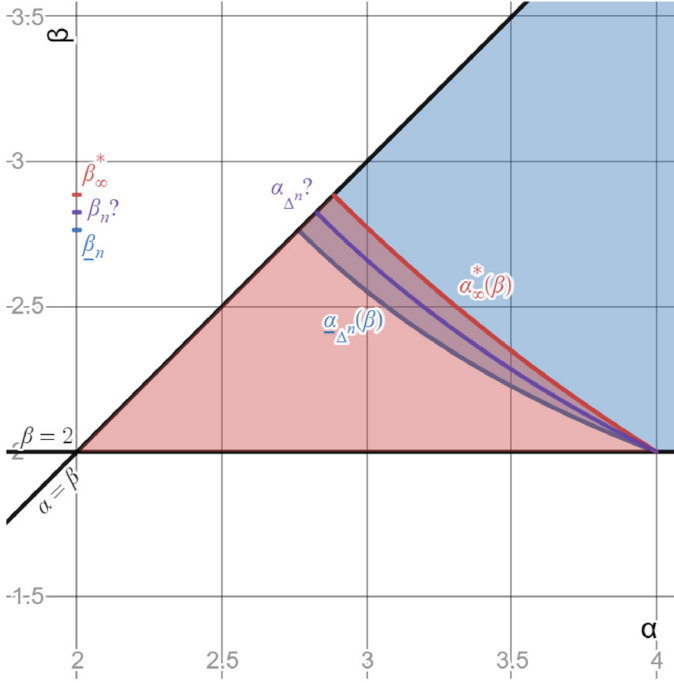
Fig. 5. The mildly repulsive regime for, e.g., n = 2 . In the red region to the left of the blue curve \alpha = \alpha_{\Delta^2}(\beta) , the simplex does not minimize \mathcal{E}_{W_{\alpha,\beta}} . Conversely, in the rightmost blue region, the simplex uniquely minimizes \mathcal{E}_{W_{\alpha,\beta}} . In the intermediate region, it is not entirely known where the simplex minimizes \mathcal{E}_{W_{\alpha,\beta}} , but the graph of the threshold function \alpha_{\Delta^2} must lie entirely in this region
