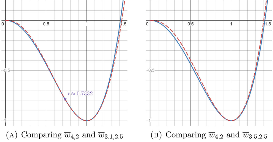
Fig. 4. Comparison of \bar{w}_{4,2} to \bar{w}_{3,1,2,5} and \bar{w}_{3,5,2,5} illustrates Lemma 4.4. Note that the unique positive root z_{\alpha,\beta} of \bar{w}_{\alpha,\beta} is ordered so that z_{3,5,2,5} = 1.4 < z_{4,2} = \sqrt{2} < z_{3,1,2,5} = \left(\frac{3.1}{2.5}\right)^{\frac{1}{3.1-2.5}} \approx 1.431 . On one hand, the proof of the lemma implies that \bar{w}_{3,1,2,5}(z_{3,1,2,5}) = 0 < \bar{w}_{4,2}(z_{3,1,2,5}) . Thus, by continuity, there exists some \varepsilon > 0 such that \bar{w}_{3,1,2,5}(r) < \bar{w}_{4,2}(r) for all r \in (z_{3,1,2,5} - \varepsilon, z_{3,1,2,5}] \approx (0.7332, 1.415] . On the other hand, the lemma implies that, since the graph of \bar{w}_{3,5,2,5} intersects the x -axis at z_{3,5,2,5} < \sqrt{2} , the inequality \bar{w}_{3,5,2,5}(z_{3,5,2,5}) \geq \bar{w}_{4,2}(z_{3,5,2,5}) extends to all r \in (0, z_{3,5,2,5}]
