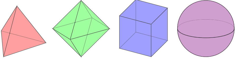
Fig. 1. Convex hulls of supports of sample minimizers of \mathcal{E}_{W_{4,2}} in \mathcal{P}_0(\mathbf{R}^3) . Each of these four minimizers is inscribed in the sphere of radius \sqrt{3}/8 and has mass uniformly distributed over the set of extreme points of the convex hull of its support. Moreover, rotates and convex combinations of any of these minimizers are also minimizers. This implies that general minimizers of \mathcal{E}_{W_{4,2}} need not have any rotational symmetries
