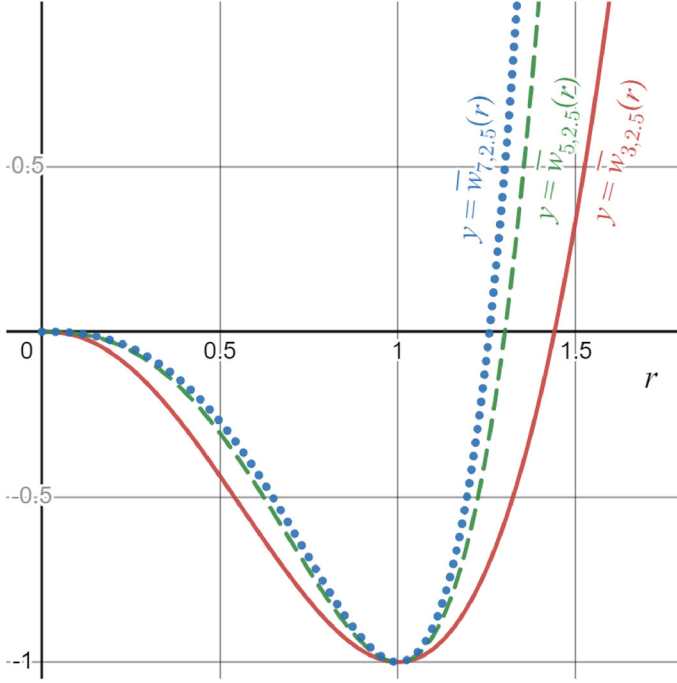
Fig. 3. Graphs of \bar{w}_{\alpha,\beta}(r) for \beta = 2.5 and \alpha = 3, 5, 7 illustrating the results of Lemma 3.1. In particular, although all three graphs agree for r \in \{0, 1\} , we see that \bar{w}_{\alpha,\beta}(r) is a strictly increasing function of \alpha for each r \in (0, 1) \cup (1, \infty) . Note that the symmetry \bar{w}_{\alpha,\beta} = \bar{w}_{\beta,\alpha} from (3.1) ensures that the monotonicity in \beta proven in Lemma 3.1 and the monotonicity in \alpha shown in this figure are equivalent
