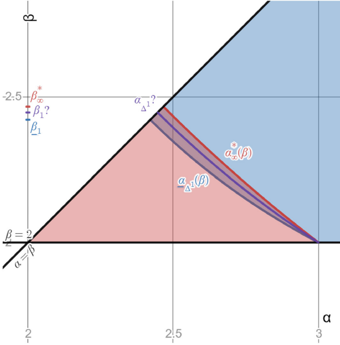
Fig. 6. The analogous graph for the n = 1 case. All coloured regions and graphs have the same meaning as their counterparts in Fig. 5, although the scale of this graph differs from its higher dimensional counterparts, due the fact that 4^* = 3 when n = 1
