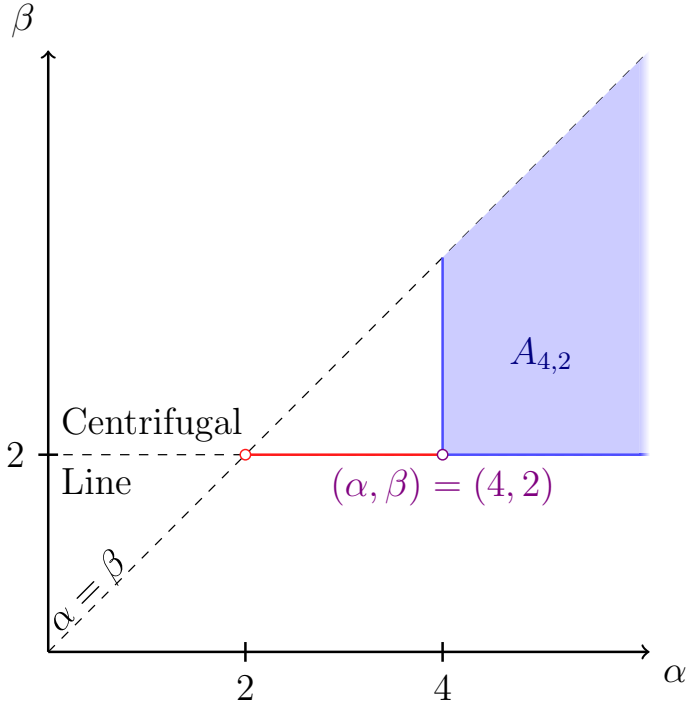
Fig. 2. Partial phase diagram of the mildly repulsive region \alpha > \beta \geq 2 for n \geq 2 : on the red segment linking (2, 2) to (4, 2) , energy is uniquely minimized by a spherical shell [17]. At (\alpha, \beta) = (4, 2) , the energy is minimized by any convex combination of the configurations described in Fig. 1, but also admits other minimizers characterized by Theorem 1.1. In the blue region, A_{4,2} , Theorem 1.2 and the fact that the balanced unit simplices \mathcal{P}_{\Delta^n} minimize \mathcal{E}_{W_{4,2}} combine to imply that the interaction energy is minimized precisely by the elements of \mathcal{P}_{\Delta^n}
